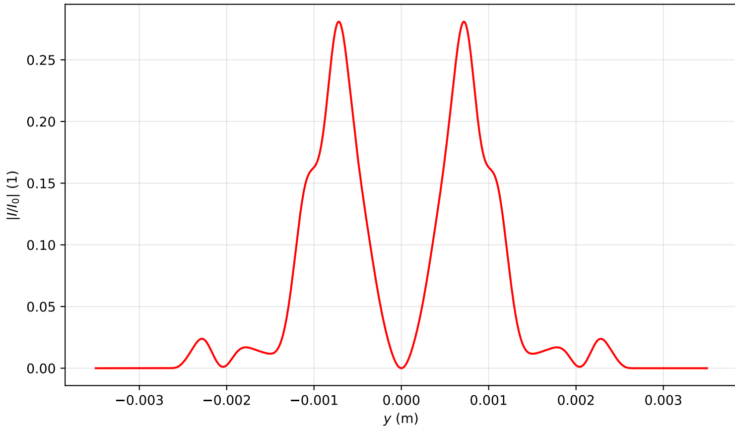
Intensity profile I(x=0, y, z=3.503)/I_0 , \text{Pin}=6.0\text{Pcr} , artificial time
